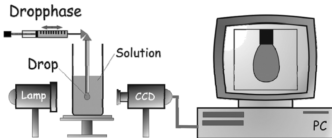
Suppl.-Figure 1. Sketch of pendant drop apparatus.
