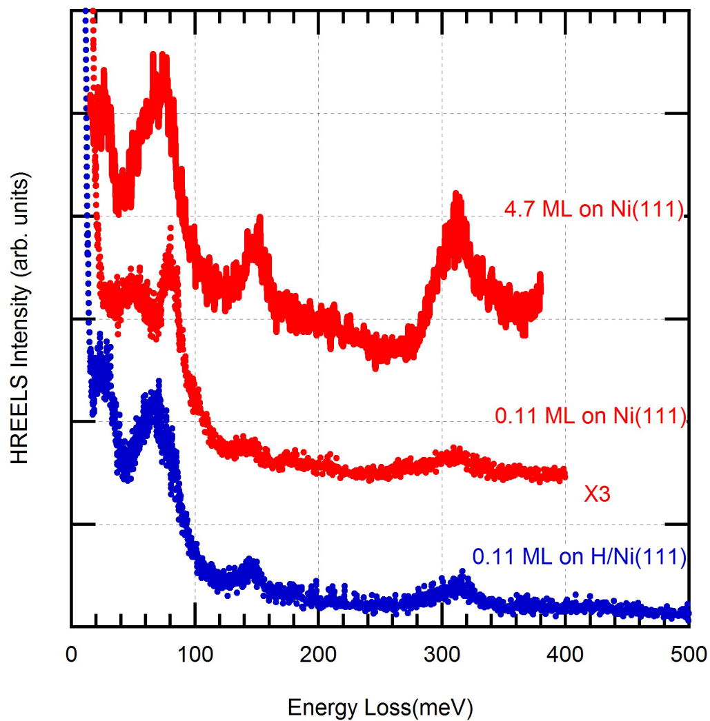
Figure 7 provides full range HREEL spectra of the traces shown in figure 5 in the text.
