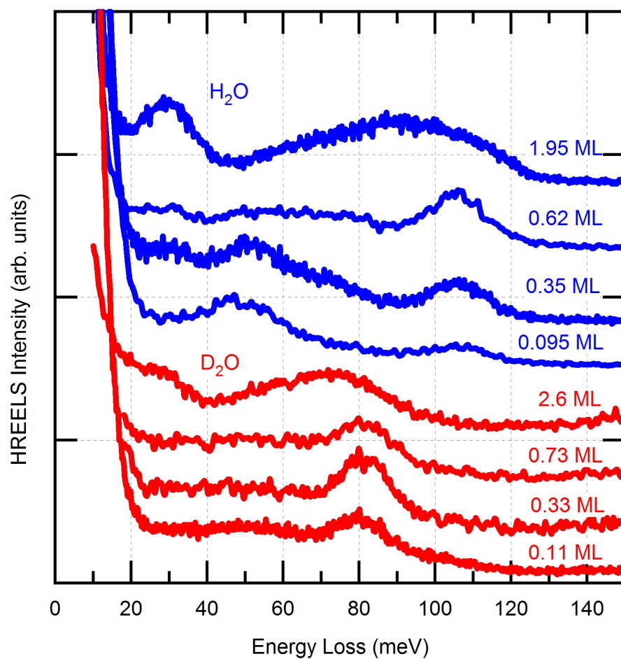
Figure 6 provides a more detailed view of the features observed in the lower energy loss regime for small doses of H 2 O and D 2 O (see also figure 5). A detailed discussion of the individual features and the interpretation are given in the text.
