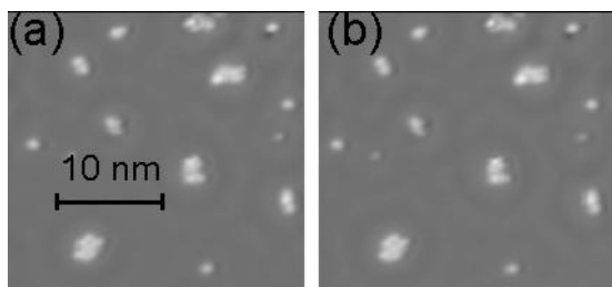
5 Fig. S1: Overview image of DCIB on Ag(111): (a) Some molecules dissociated upon adsorption or cluster into larger islands (b) same spot of the surface imaged seven minutes 10 after (a) showing that molecules are stationary at 5K; small shift of all molecules by to the right originates from a small thermal drift.
