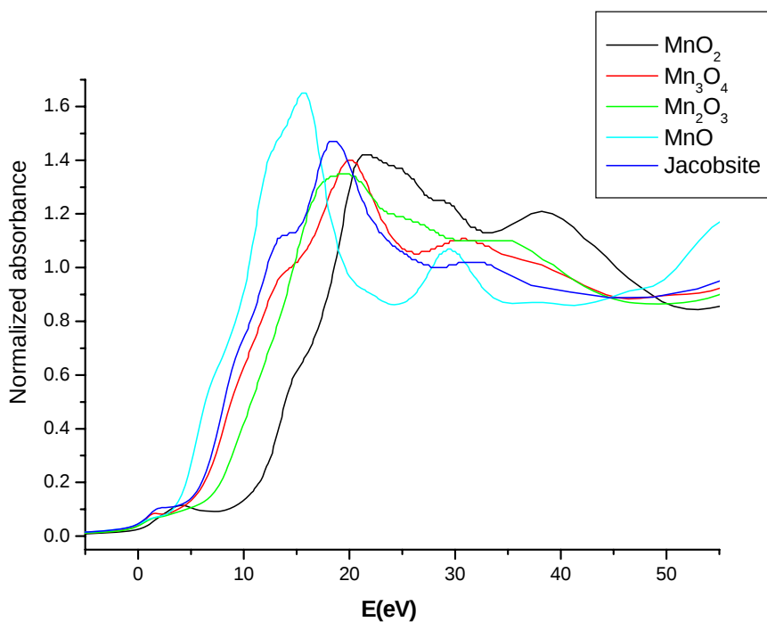
Fig. S2: XANES spectra at the Mn K-edge of standards
