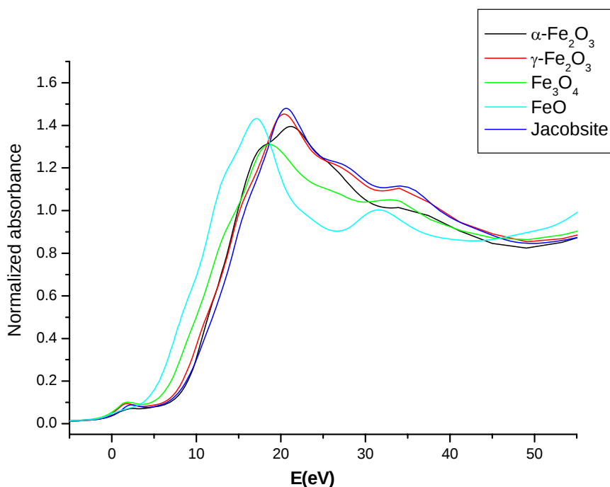
Fig. S1: XANES spectra at the Fe K-edge of standards
