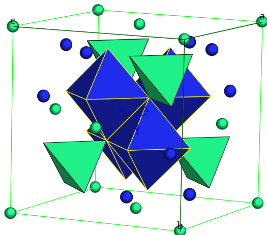
Fig. S3: Scheme of a spinel structure showing the octahedral and tetrahedral units.
