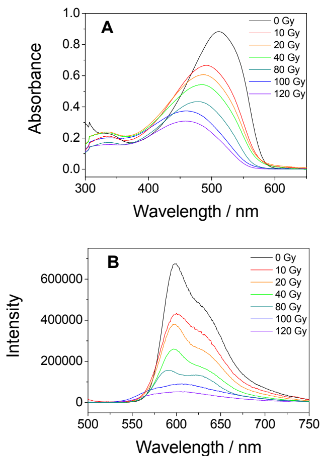
Figure S1. Absorption (A) and PL (B) spectra of MEH-PPV/DIB (1:30) composite films before and after \gamma exposure (0-120 gray)
