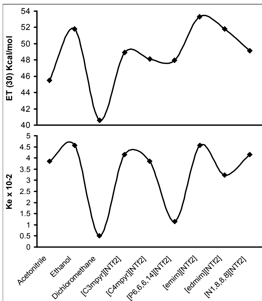
Figure S1. Correlation between K_e and E_T(30) values in molecular solvents and ionic liquids.
