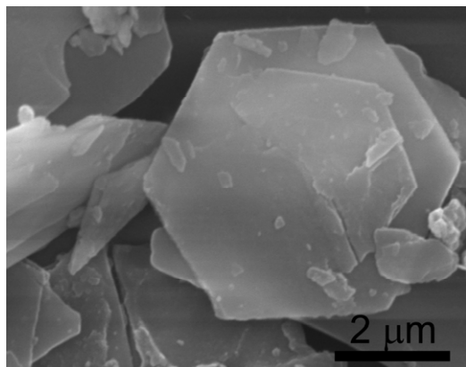
Figure S1. The SEM image of the as-prepared Co-Al LDH.
