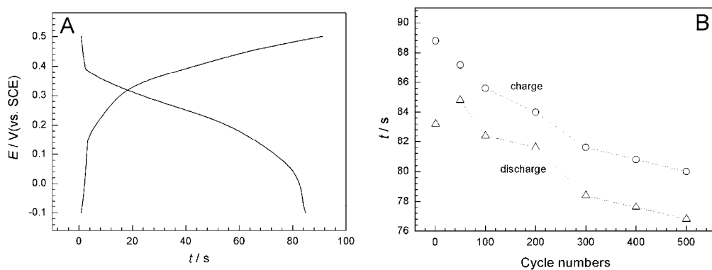
Figure S2. The charge/discharge curves (A) and long-term performance (B) of the Co-Al LDH at the constant current density of 2 \text{ A g}^{-1} in the solution of 1 \text{ M KOH} + 0.05 \text{ M K}_3\text{Fe}(\text{CN})_6 + 0.05 \text{ M K}_4\text{Fe}(\text{CN})_6 .
