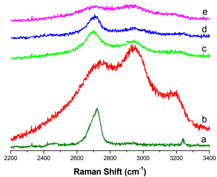
SI 1. Second-order Raman spectra of (a) Gr, (b) GO, (c) GN1, (d) GN2 and (e) GN3.
