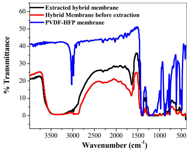
Figure S1. Representative FTIR spectra of hybrid membranes with additional SBA-15-SO 3 H powder (before and after extraction of the surfactant and PVDF-HFP membrane as reference).
