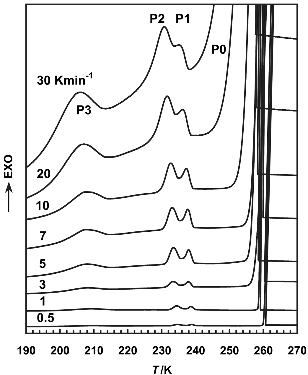
Supple. Fig. 1. Effect of scanning speed on the DSC curves, MCM-41 C12.
