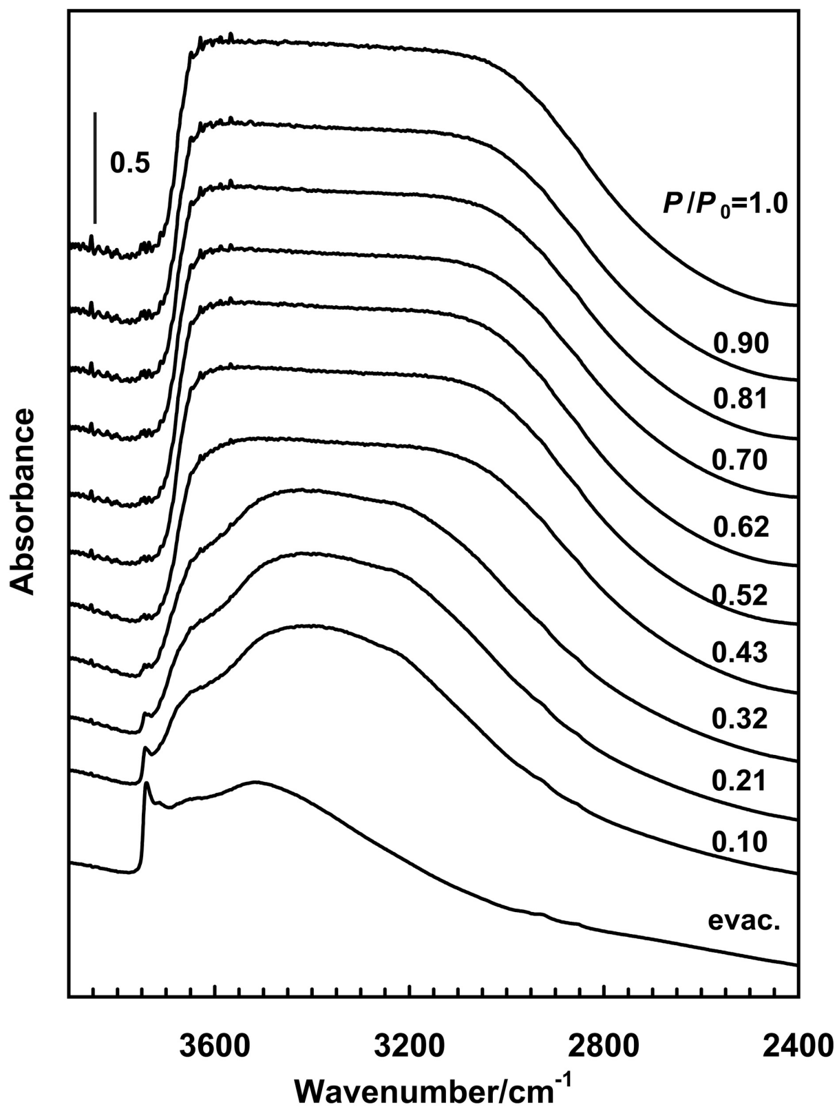
Supple. Fig. 2. Effect of adsorption of water on the OH stretching band, MCM-41 C12
