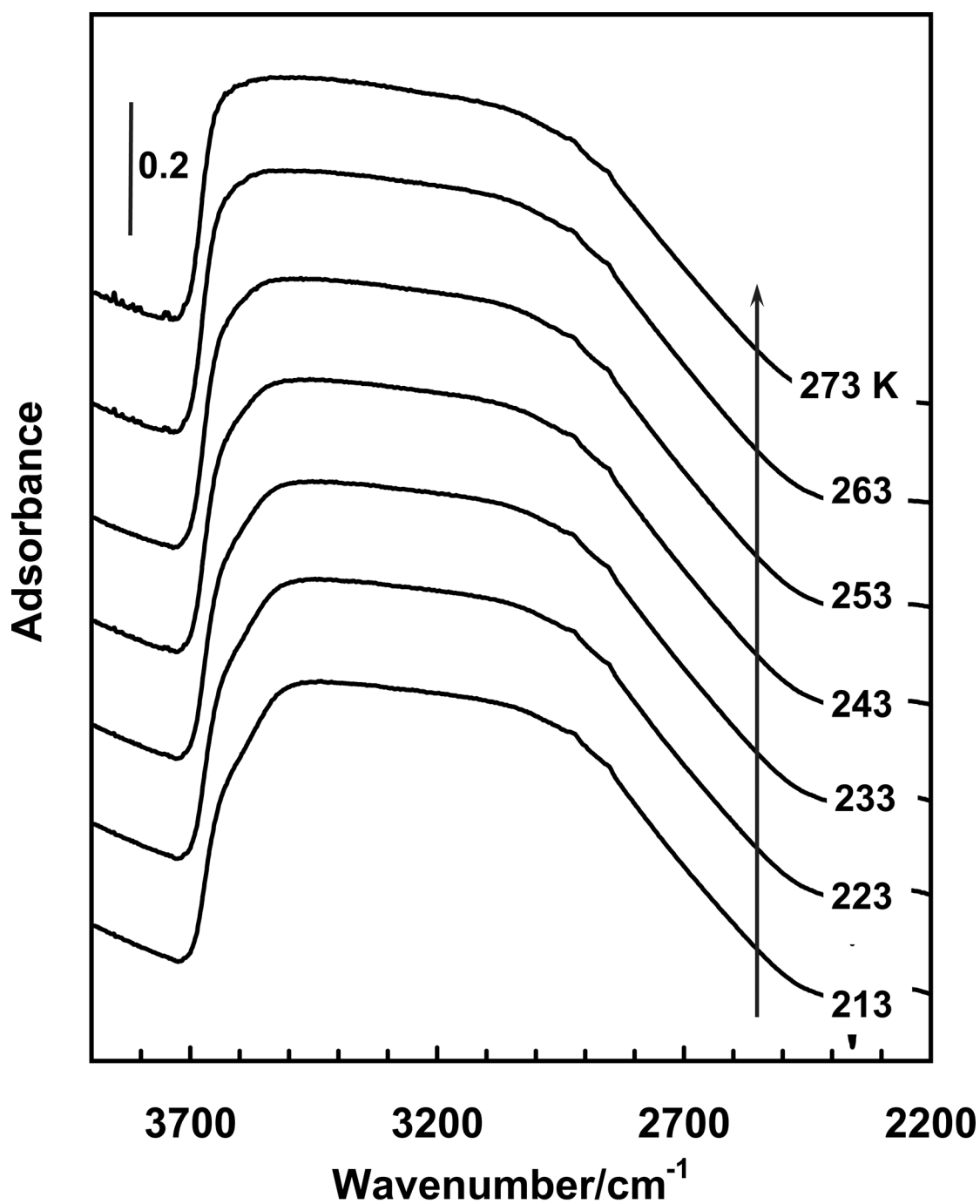
Supple. Fig. 3. FTIR spectra of water confined in MCM-41 C12 determined at increasing temperatures.
