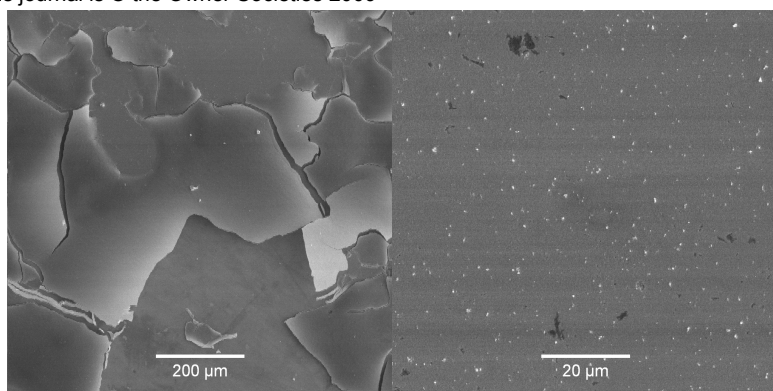
Fig 1 SEM images of CdS films prepared on bare FTO (left) and plasma treated FTO (right)
