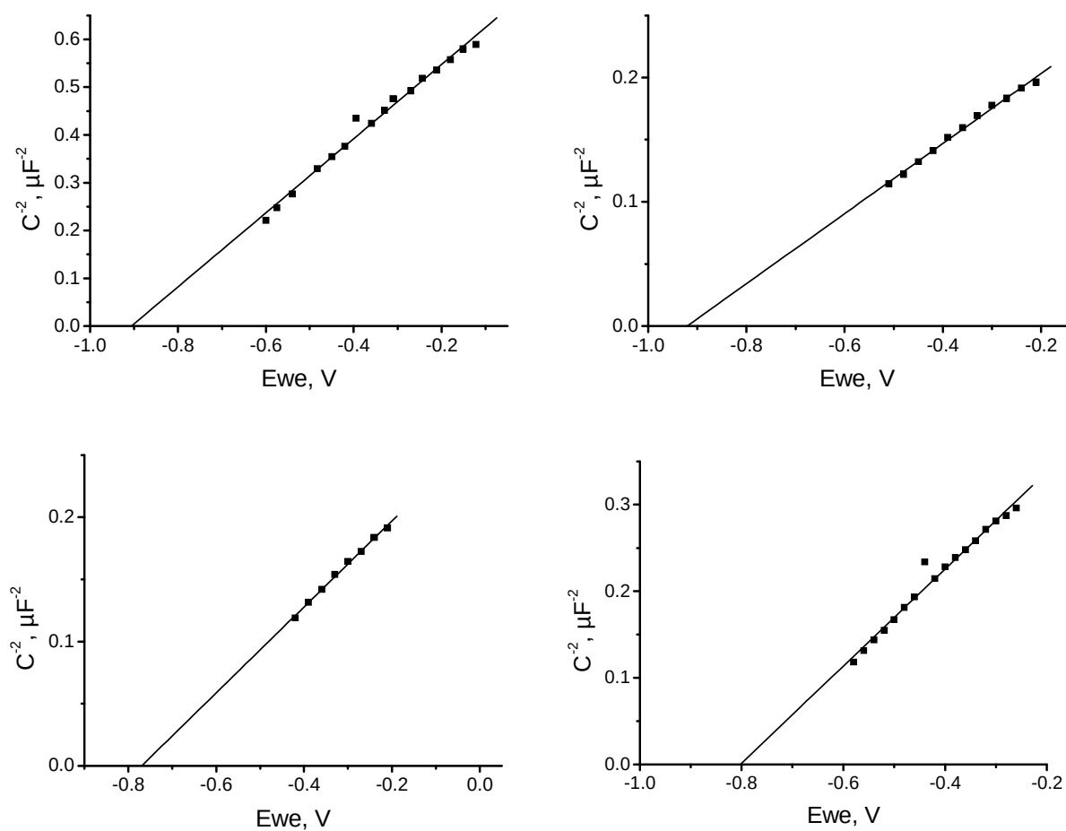
Fig 2 Mott-Shottky plots of electrodeposited CdS films on plasma treated FTO in 0.1M Na 2 S and 0.1M NaOH at 1kHz.
