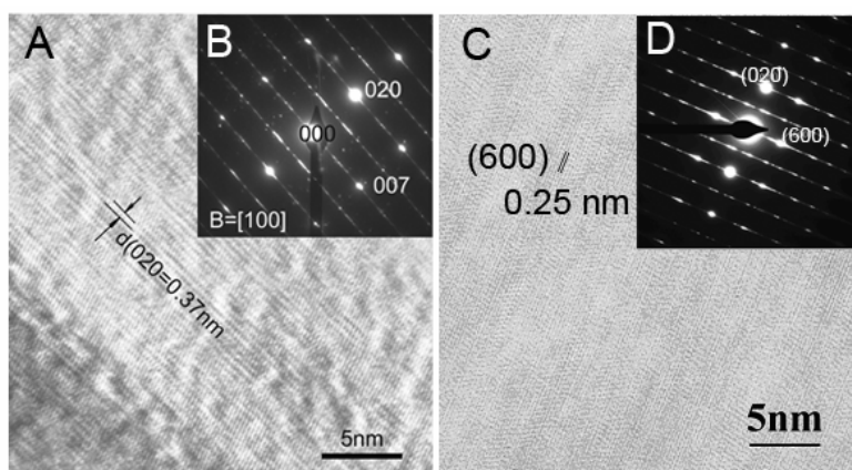
Figure S1. HRTEM images and electron diffraction patterns of T3 (A, B) and T6 (C, D) nanofibers.
