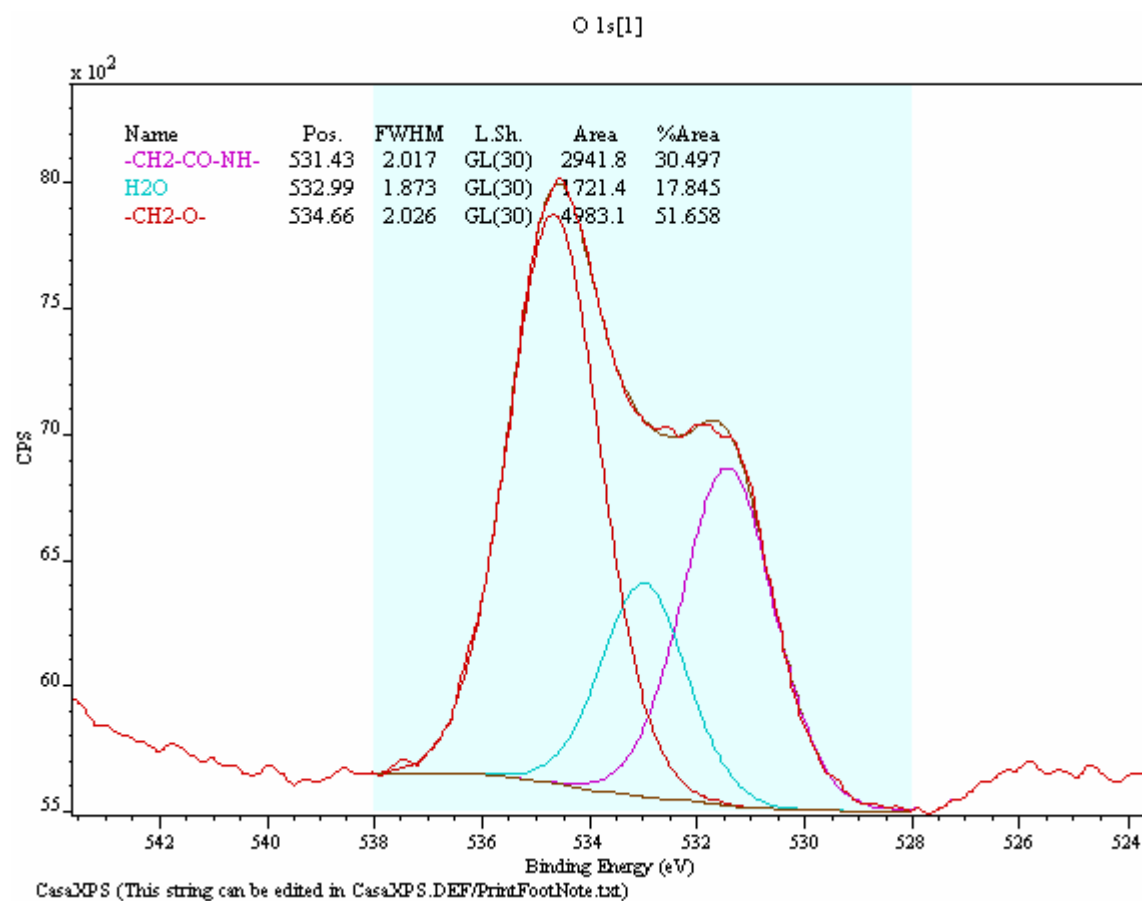
Figure SI 1b: Core level XPS spectra of Au-MEODA for O (1s).
