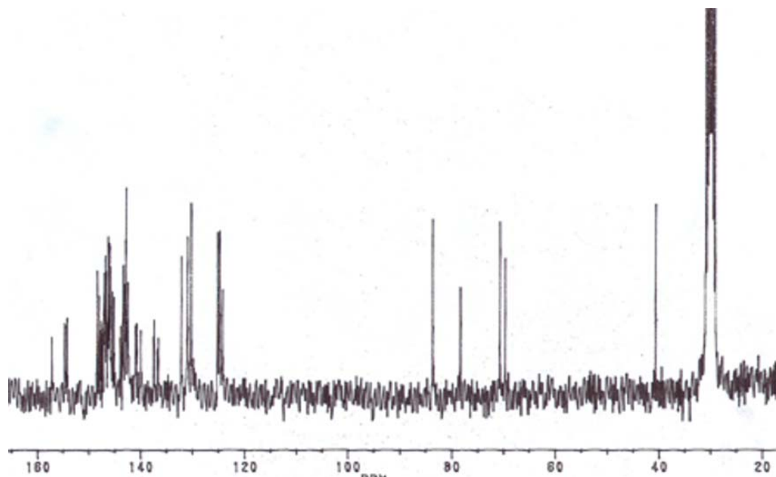
Figure S2. ^{13}\text{C} -NMR spectrum of bis-fullerene 3 .
