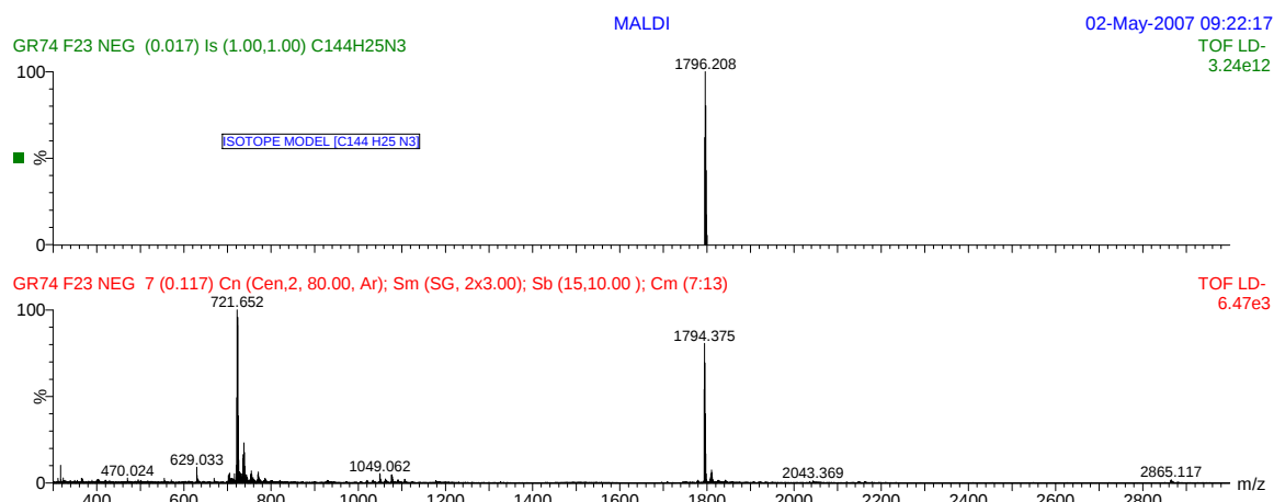
Figure S4. MALDI-TOF MS spectrum of bis-fullerene 3 .
