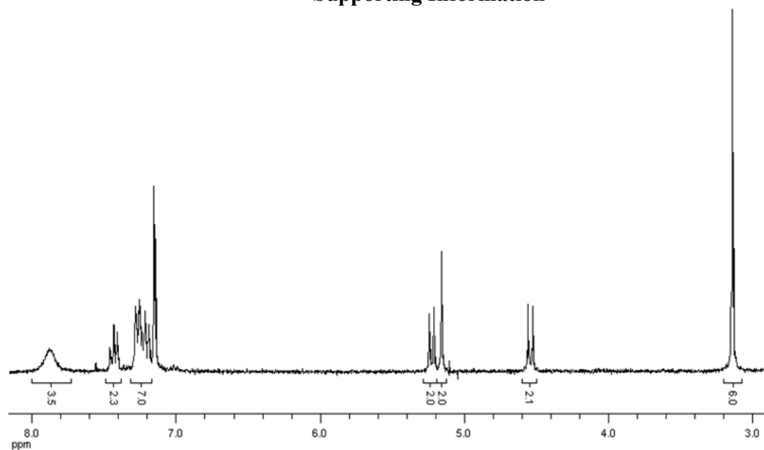
Figure S1. ^1\text{H} -NMR spectrum of bis-fullerene 3 .
