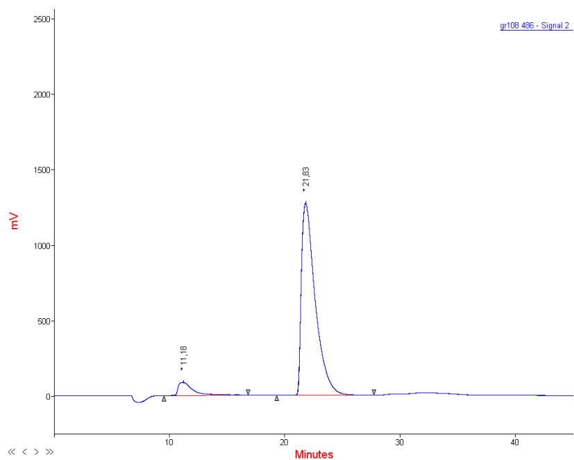
Figure S3. HPLC chromatogram of silica gel column fraction containing bis-fullerene 3 (retention time: 21.83 min).
