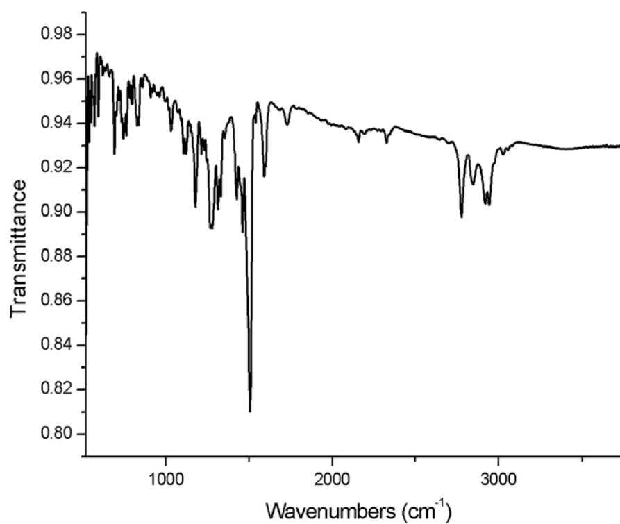
Figure S5. ATR-IR spectra of bis-fullerene 3 .
