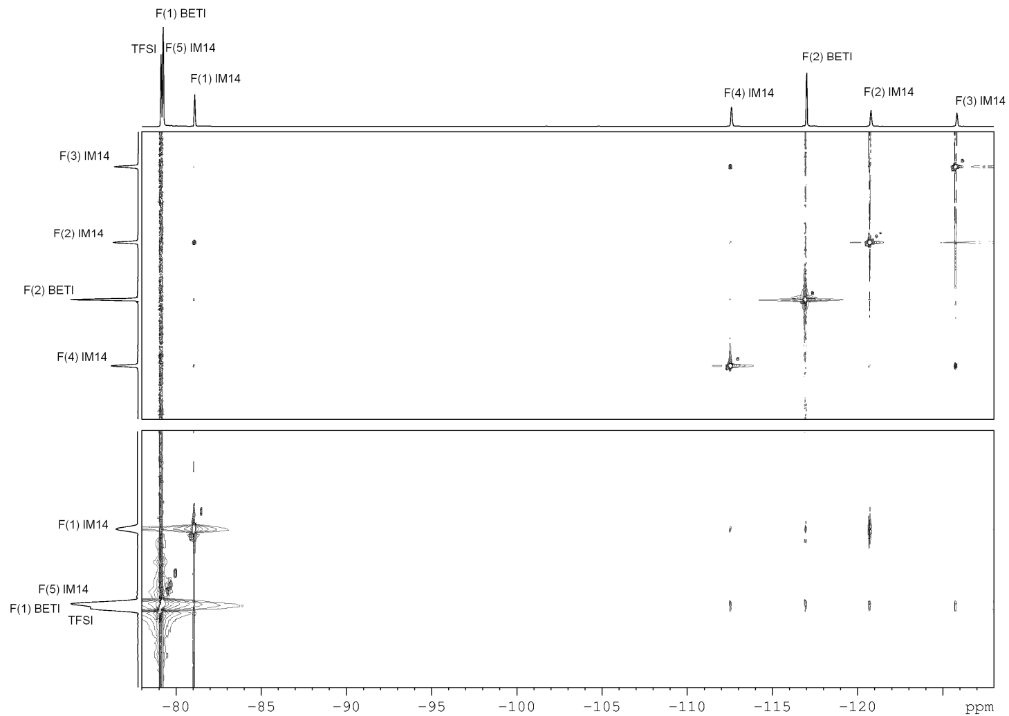
Figure S3. ^{19}\text{F} - ^{19}\text{F} NOESY spectrum of ABC mixtrure
