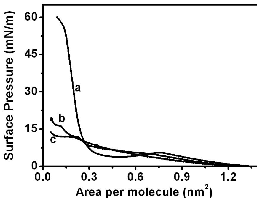
Fig. S1. Surface pressure-area isotherms of 2-AGE monolayers: (a) without UV irradiation, (b) in situ UV irradiating in the monolayer, and (c) spreading film from the photo-irradiated solution.
