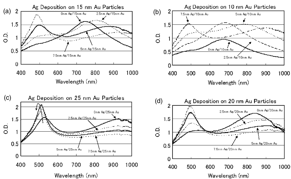
Figure S2. Spectra of most spots for the combinatorial particle array shown in Fig. 12. With thinner gold deposition thicknesses, even a very thin silver deposition has a large effect in the resulting spectrum.
