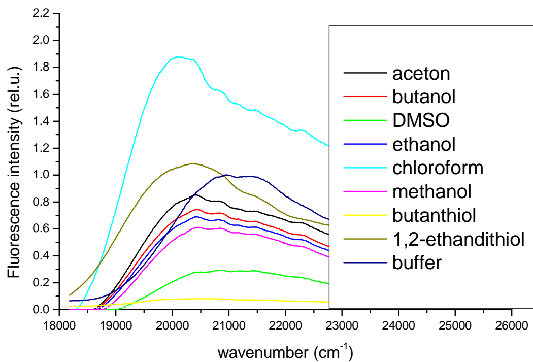
Figure S4 Excitation spektrum of SG + in various solvents.
