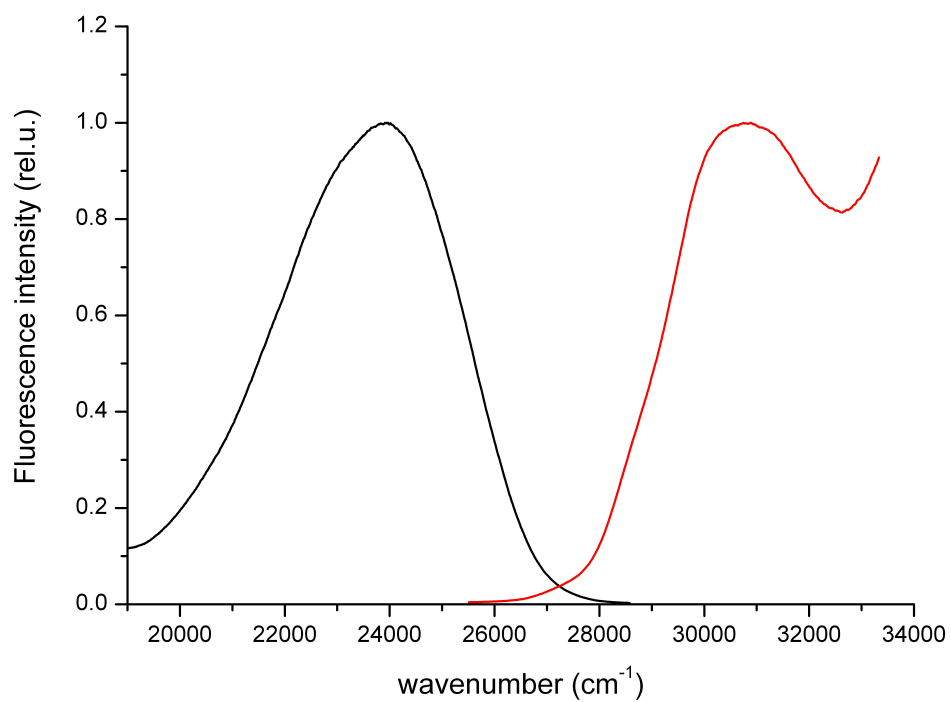
Figure S1 Excitation (red) and emission (black) spectrum of SGOH.
