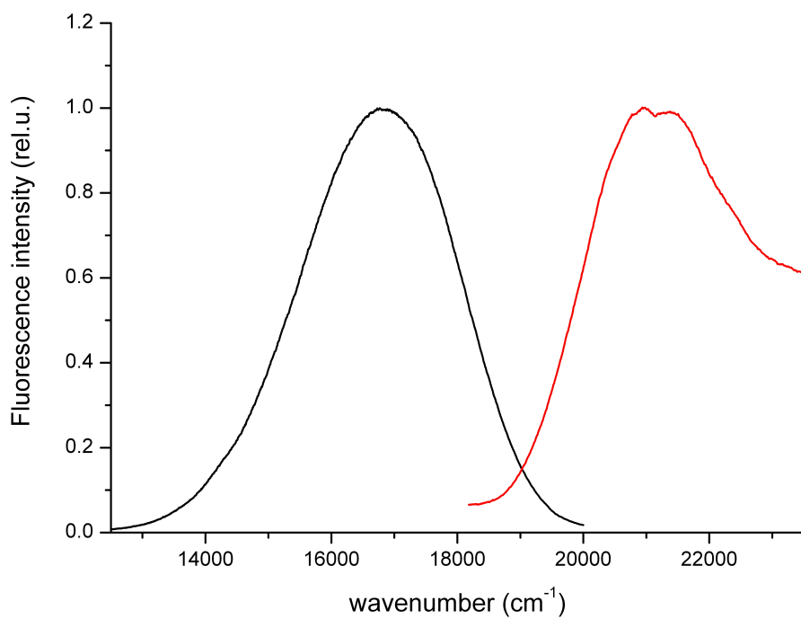
Figure S2 Excitation (red) and emission (black) spectrum of \text{SG}^+ .
