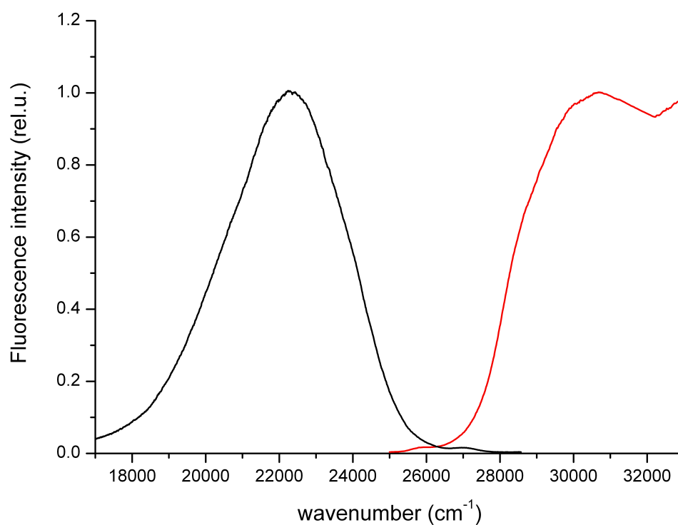
Figure S3 Excitation (red) and emission (black) spektrum of DHSG.
