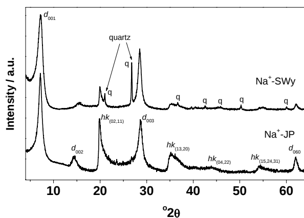
Figure ESI 1. X-ray diffraction patterns of \text{Na}^+ -JP and \text{Na}^+ -SWy samples
