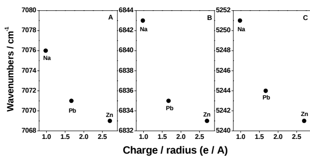
Figure ESI 2. The position of A) 2\nu_{\text{H}_2\text{O}} , B) 2\nu_{\text{W}} , and C) (\nu+\delta)_{\text{H}_2\text{O}} bands as a function of ionic charge/radius ratio for \text{Na}^+ -, \text{Pb}^{2+} -, and \text{Zn}^{2+} -JP
