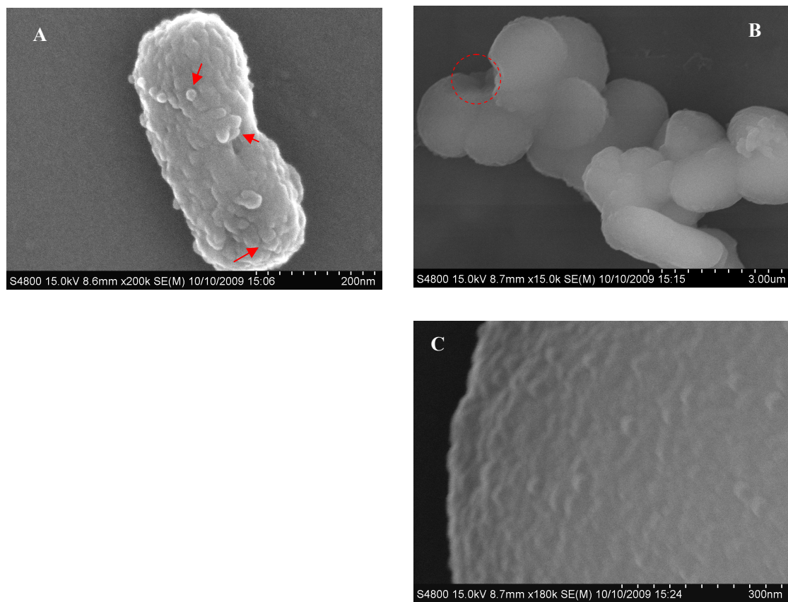
Figure S4 SEM images of vinyl-functionalized PMOs based on BTEB/TEVS. (A) TEVS-15; (B) TEVS-60; (C) magnified (B).
