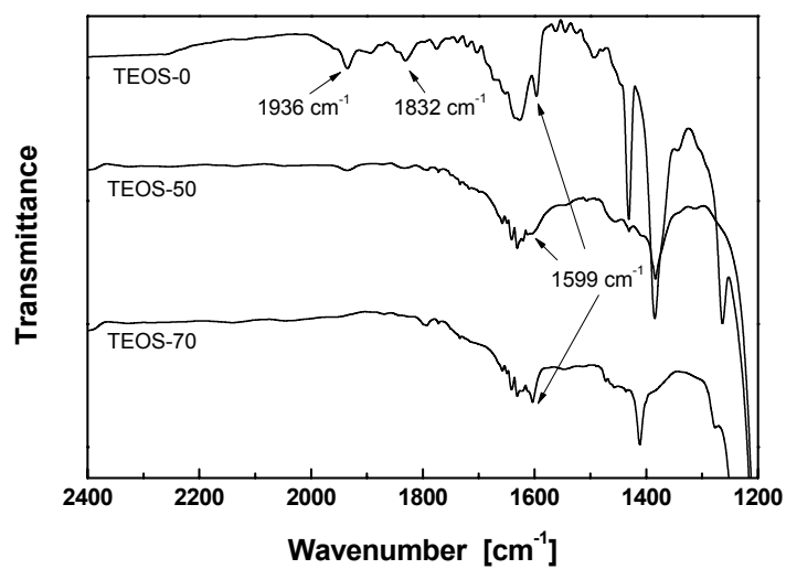
Figure S2 FTIR spectra of vinyl-functionalized PMOs based on BTEB/TEOS/TEVS with various molar percentages of TEOS.
