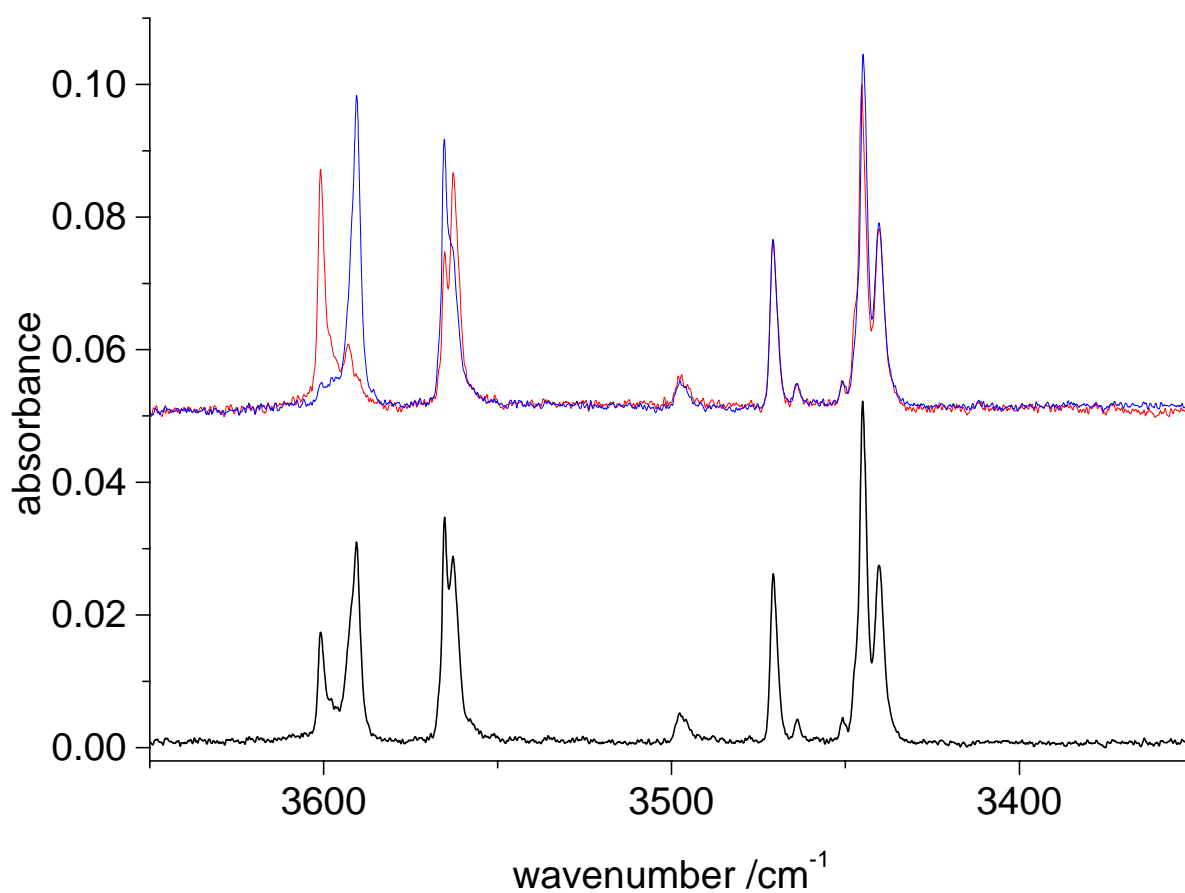
Figure S1. Mid-IR spectra of cytosine isolated in an Ar matrix: (black) recorded after deposition of the matrix; (red) after irradiation at 7013\text{ cm}^{-1} ; (blue) after irradiation at 7034\text{ cm}^{-1} .
