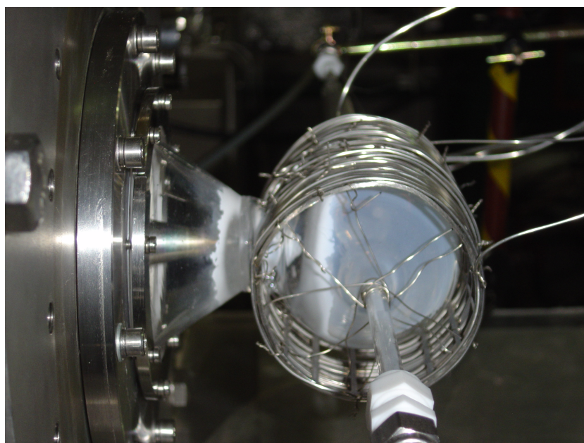
Figure S2. Photography of the reactor used in Hefei with a part of the heating resistances and connected to the differential pumped chamber.
