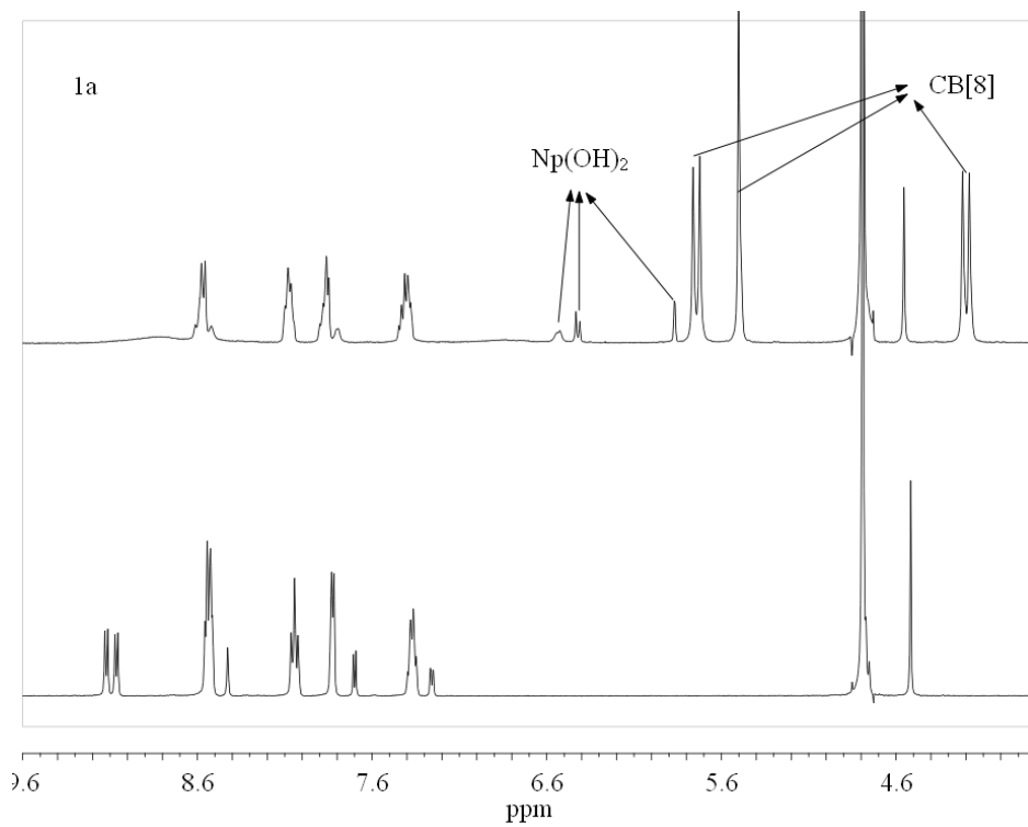
Figure S1 1 H NMR spectra (400 MHz, D 2 O) of complex 1a alone (down), after addition of 1 equiv of CB[8] and 1 equiv of Np(OH) 2 (up).
