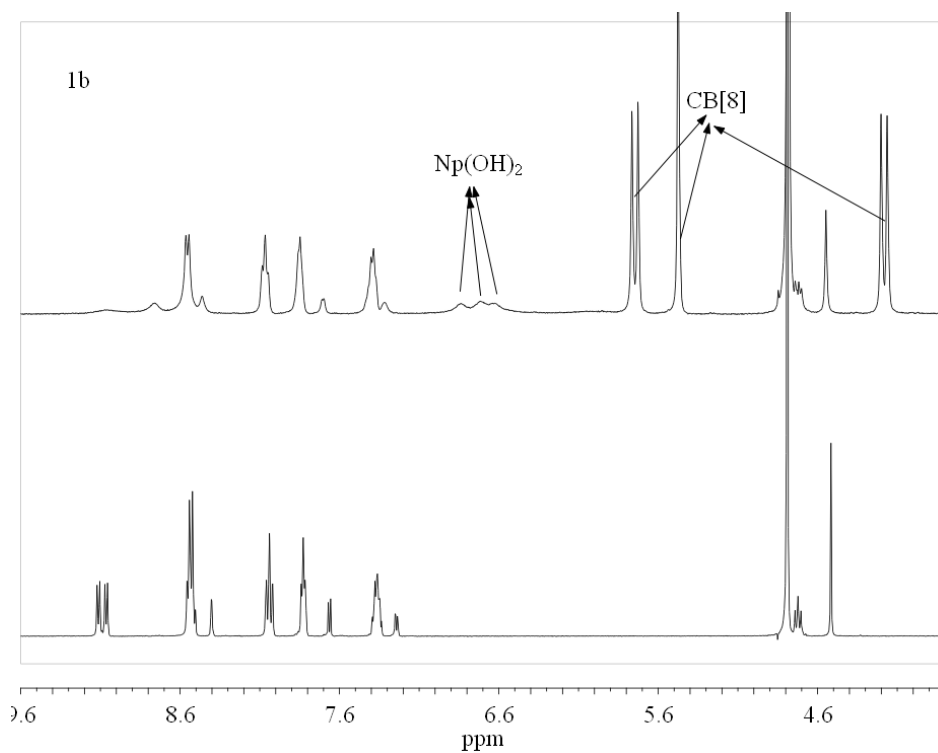
Figure S2 1 H NMR spectra (400 MHz, D 2 O) of complex 1b alone (down), after addition of 1 equiv of CB[8] and 1 equiv of Np(OH) 2 (up).
