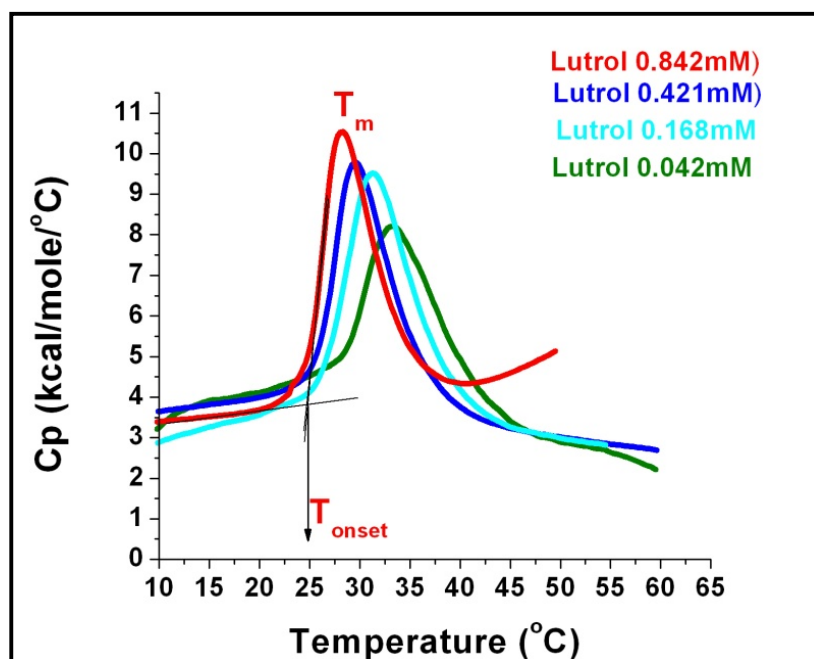
Fig. S1. Determining Lutrol CMT as a function of concentration.
