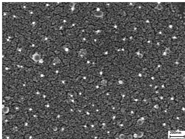
Fig S1. FESEM image of a hybrid film prepared from \text{HAuCl}_4 loaded block copolymer solution/ titania sol-gel precursor after removing the copolymer matrix. It is clearly seen that Au particles (lighter parts) form on the surface of titania.
