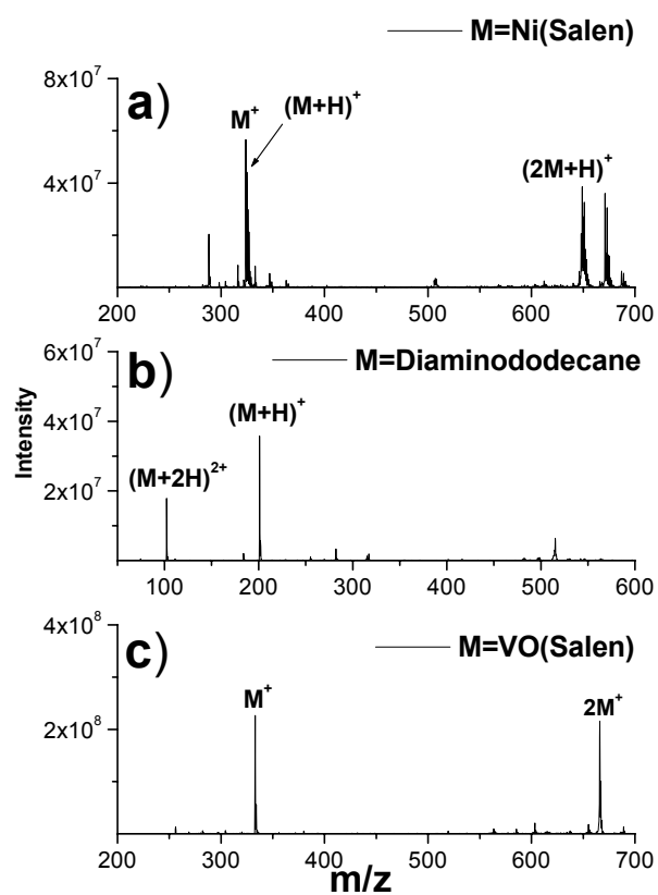
Figure S1 ESI mass spectra of (a) Ni(salen); (b) diaminododecane; and (c) VO(salen).
