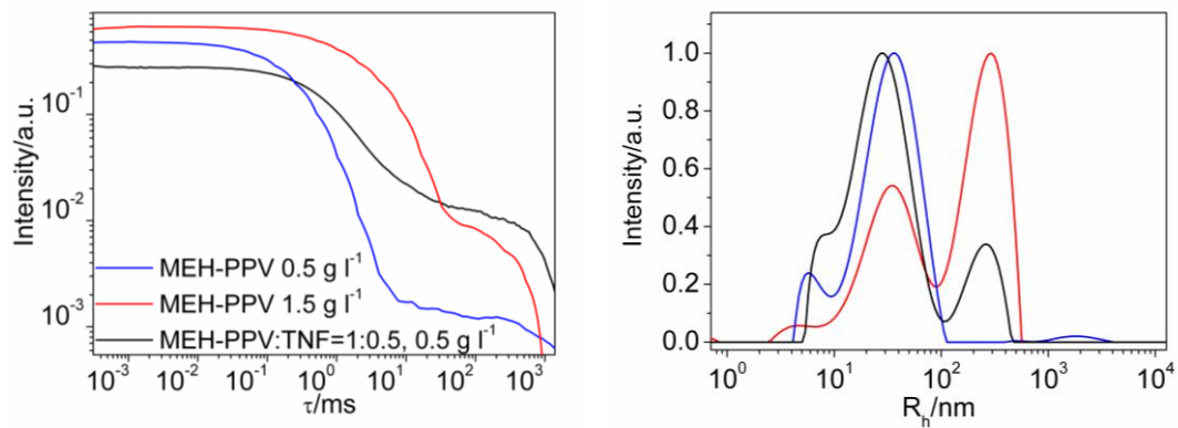
Figure 1S. The ACFs (a) and the corresponding RTDs (b) for MEH-PPV:TNF=1:0.5 dilute blend and pristine MEH-PPV solutions for various concentration. The scattering vector for all ACFs was q = 0.01 \text{ nm}^{-1} ( \theta=40^\circ ).
