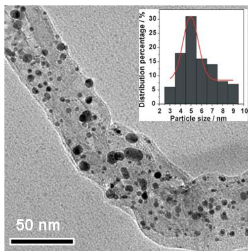
Figure S2. TEM images and histograms of Pd/acid treated-MWCNTs with Pd loading of 20wt%.
