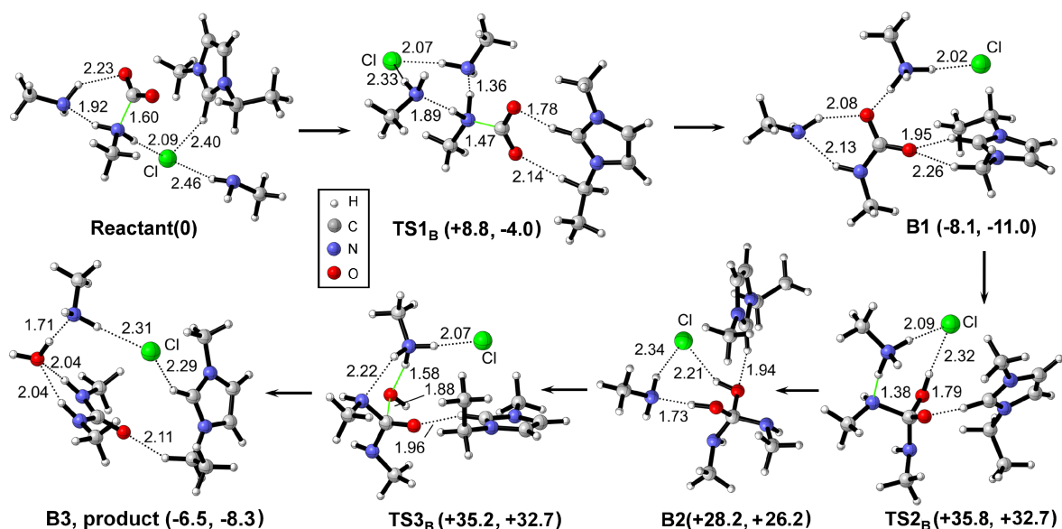
Figure 5S. Optimized structures for the interactions of methyl amine with CO 2 in the presence of [EMIm]Cl.
