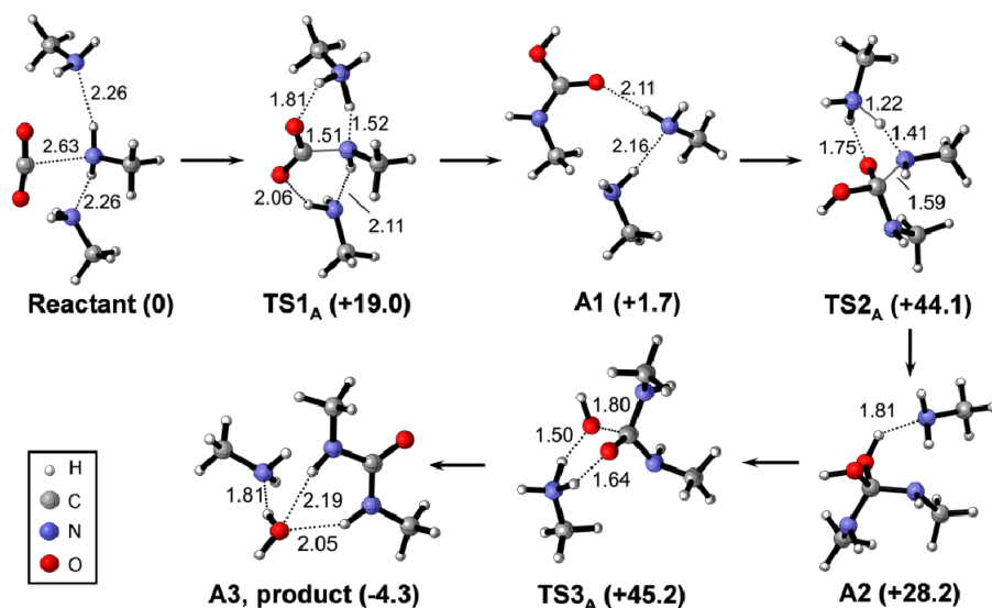
Figure 4S. Optimized structures resulting from the interactions between CO 2 and methyl amine in the absence of an IL.
