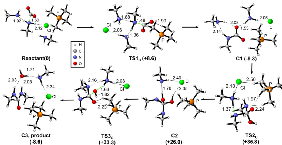
Figure 6S. Optimized structures for the interactions of methyl amine with CO 2 in the presence of Me 4 PCl.
