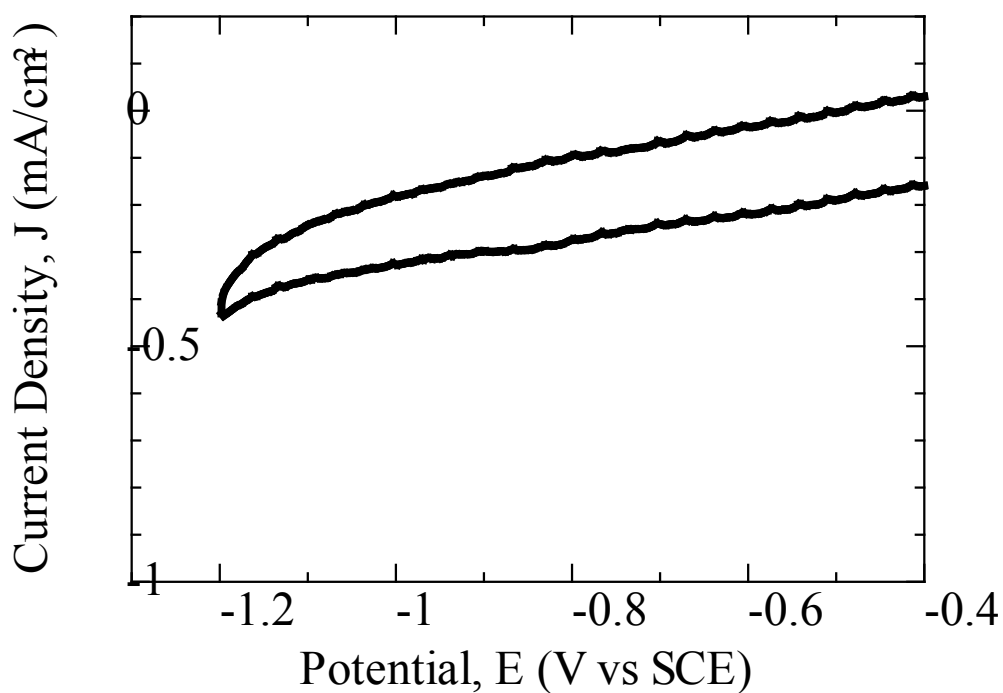
Figure S1. Cyclic voltammetric curves of as-dealloyed nanoporous Au samples without SAM. The electrolyte used was 0.1 M NaOH and the scan rate was 5 mV/s.
