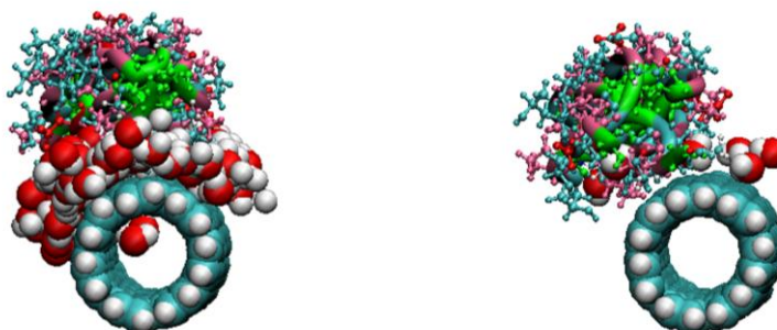
Fig. S2 GDO-CNT cross section view of initial and final conformation.
