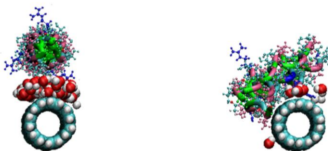
Fig. S5. GRO-CNT cross section view of initial and final conformation.
