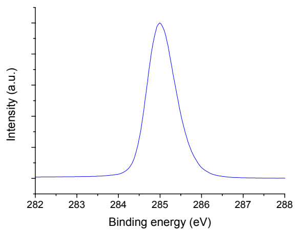
C 1s XPS spectrum of the CVD diamond reference
