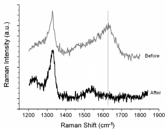
Detonation NDs Raman spectra before (top) and after (bottom) hydrogen plasma treatment.
