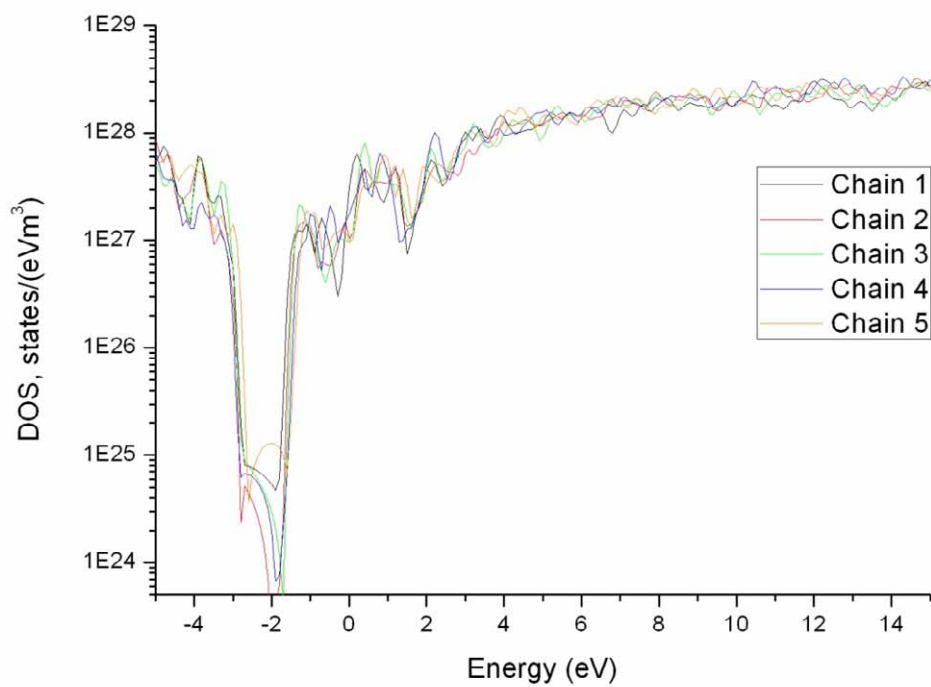
Figure 1S. Dependence of density of states (states/eVm 3 , logarithmic scale) on energy for each of the oligomers composing the amorphous system.
