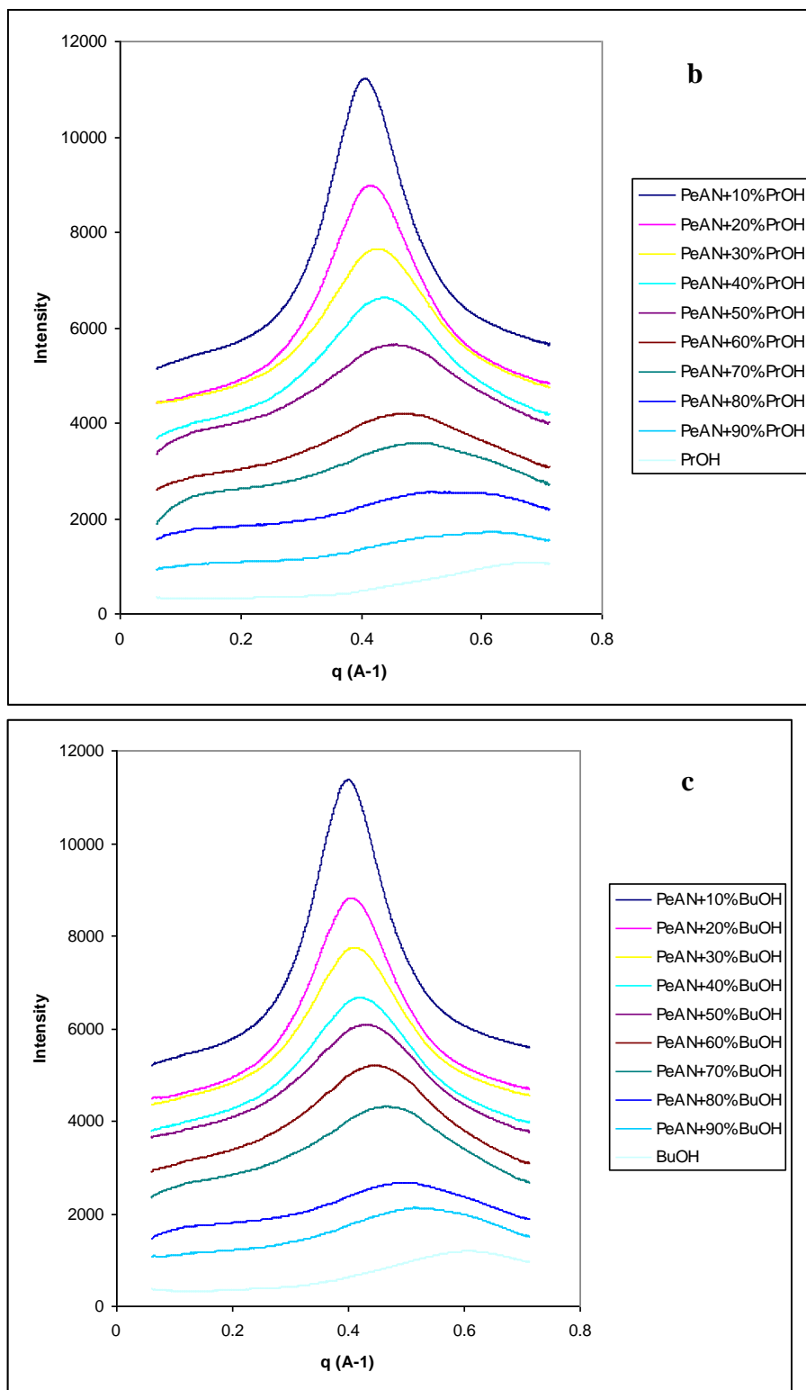
Figure S2. SAXS/WAXS patterns for PeAN showing changes to peak 1 with addition of a) ethanol, b) propanol and c) butanol. Traces have been offset to aid in viewing.
