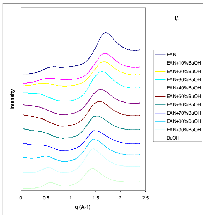
Figure S1. SAXS/WAXS patterns for EAN with addition of a) ethanol, b) propanol and c) butanol. Traces have been offset to aid in viewing.
