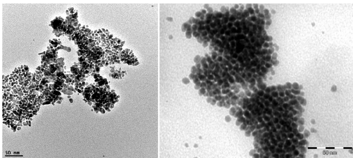
Figure S1. TEM images of NP2-dba (left) and NP-dba (right).
