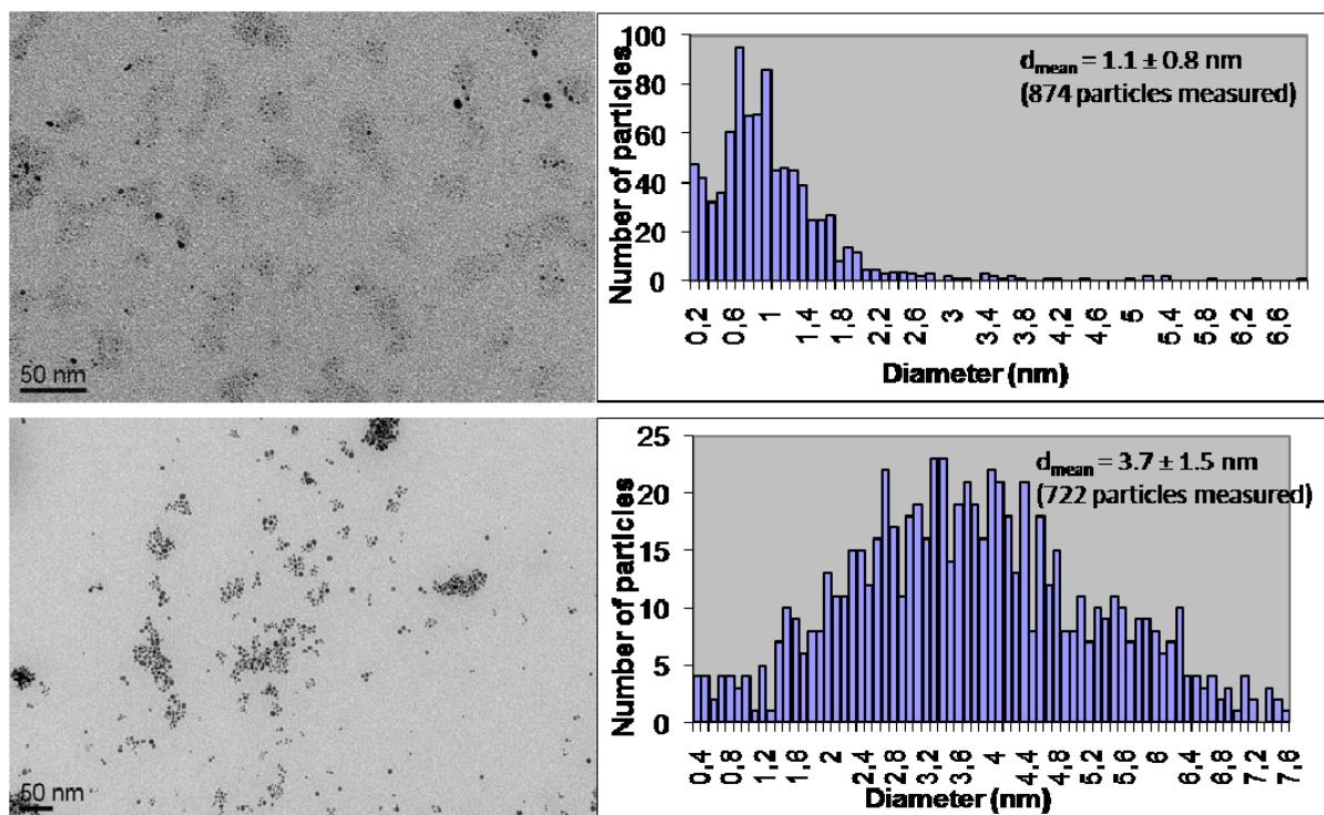
Figure S2. TEM images of particles generated in situ from palladium acetate in [EMI][MeHPO 3 ] at 100 °C (top) and after catalytic reaction of iodobenzene and butenone (bottom).
