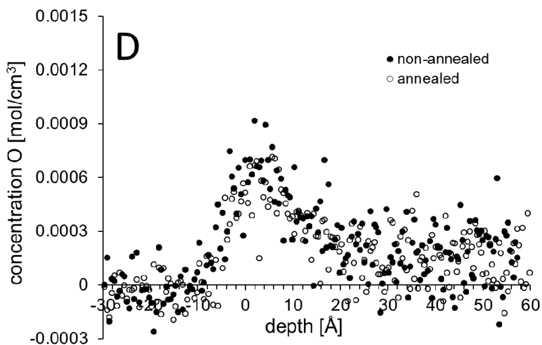
Figure 1S: Concentration depth profiles of A) sulphur and B) oxygen of the 40:60 P3HT:PCBM blend and concentration depth profiles of C) sulphur and D) oxygen of the 60:40 P3HT:PCBM blend.
