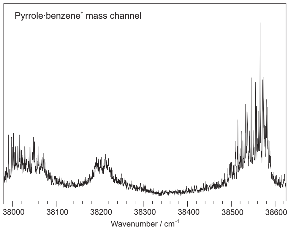
FIG. 1. One-color resonant two-photon ionization spectrum measured in the pyrrole-benzene mass channel.
