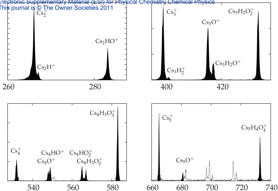
Figure 1.2: Photoionization mass spectrum of mixed \text{Cs}_k\text{H}_m\text{O}_n clusters in helium nanodroplets [4] (detailed views). Abscissa: Ion mass [amu]. Ordinate: Photoionization yield [arb. u.]. Axis ticks in all plots are equidistant. Filled and labelled peaks correspond to clusters calculated in this work.
