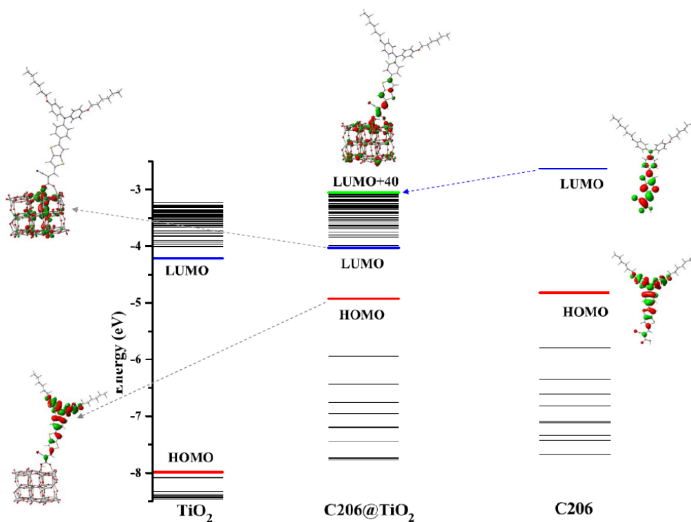
Fig.S1 Schematic energy diagram of the non-interacting and interacting C206 dye and the (TiO 2 ) 46 complex.
