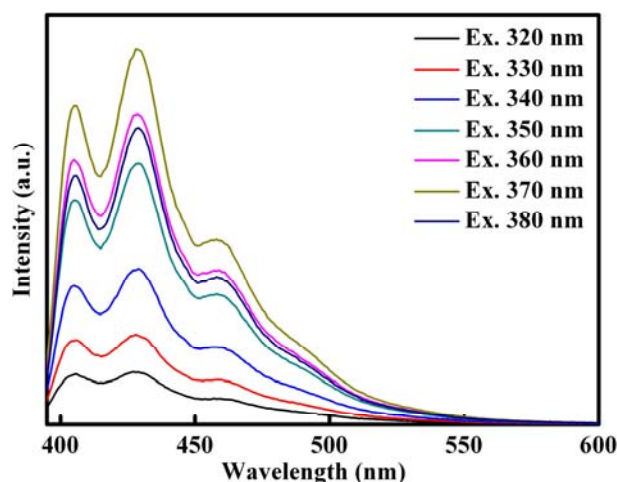
Fig. 1 Emission spectra of silicon nanocrystals synthesized by Femtosecond Laser Ablation in 1-hexene dissolved in ethanol.
