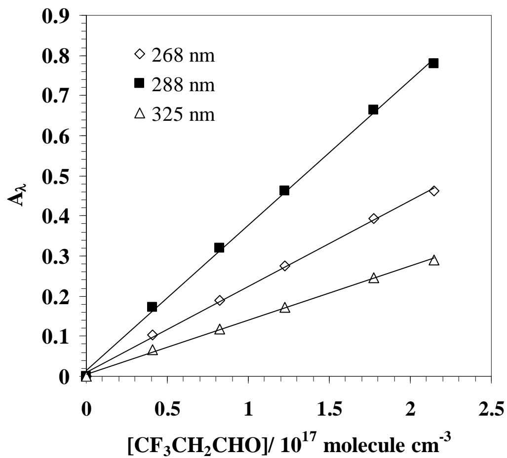
Fig.S1. Beer-Lambert law plots obtained at three different wavelengths at 298 K.
