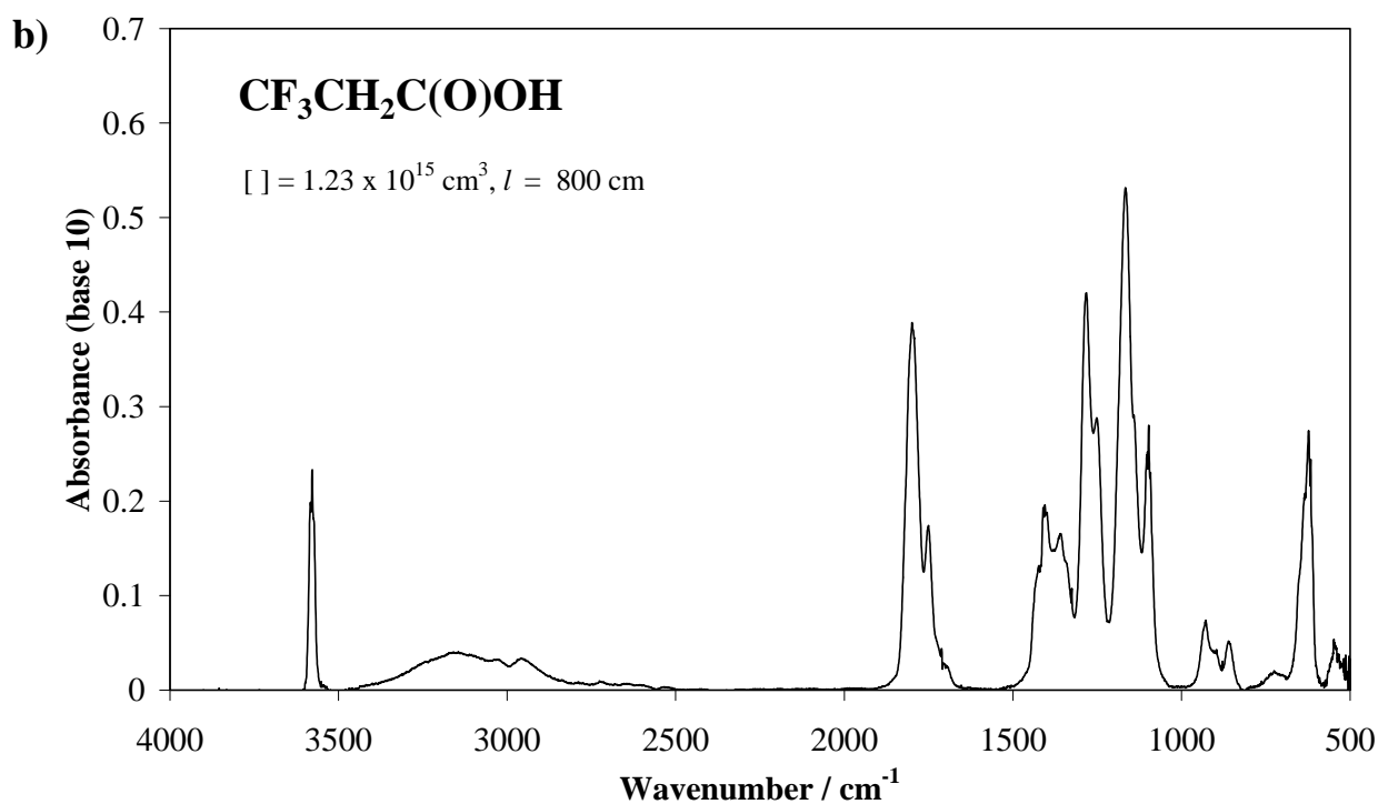
Figure S3. a) Infrared spectrum of CF 3 CH 2 OH recorded in this work together with that reported by Sellevåg et al. (2004); b) CF 3 CH 2 C(O)OH
