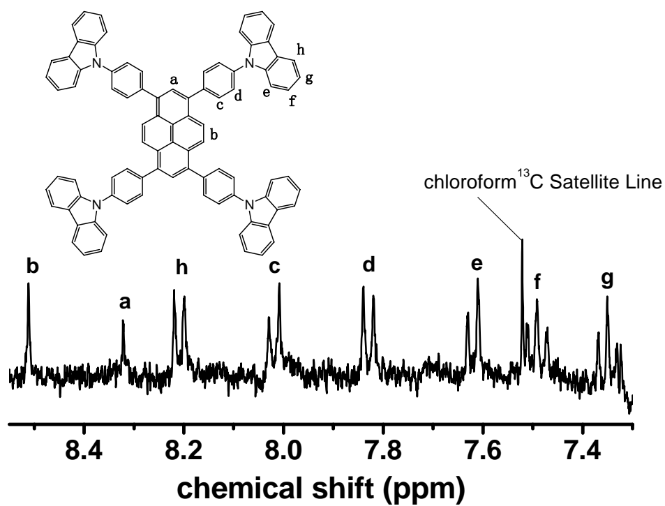
Fig. 1S. ^1\text{H} NMR spectrum of P1 in chloroform-d.
