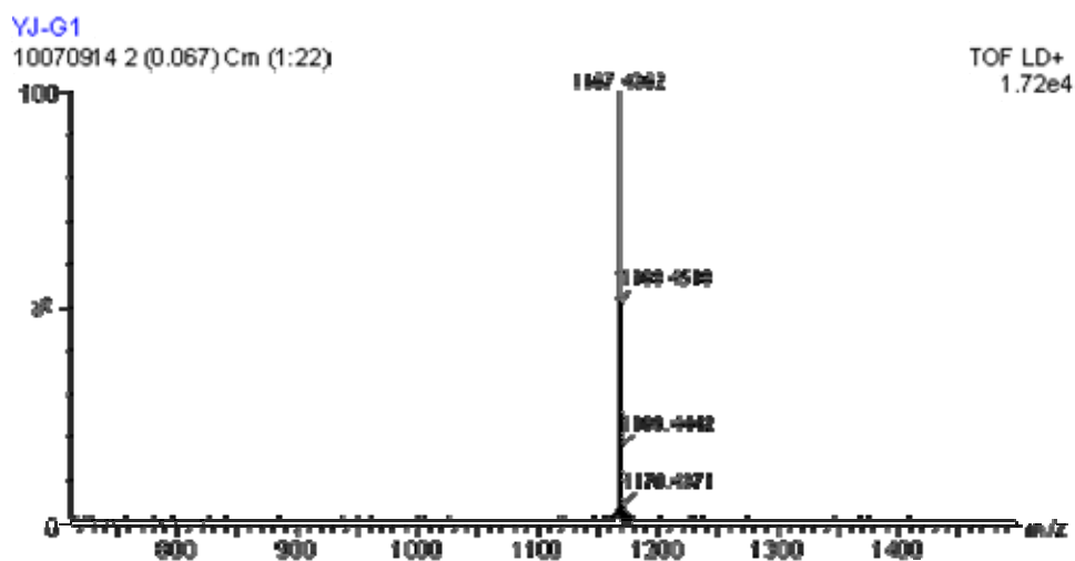
Fig. 2S. MALDI-TOF-MS spectrum of dendrimer P1.
