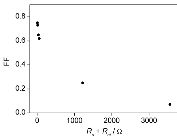
Fig. S2 A plot of FF vs. the total resistance.
