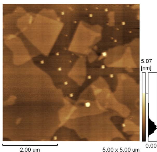
Fig. S1 A tapping mode AFM image of graphene nanosheets deposited on mica by self-assembly.
