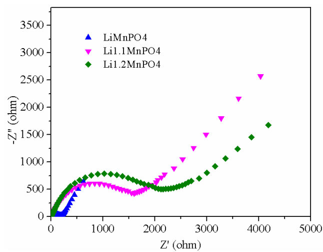
Figure S2. Comparison of the AC impedance of \text{LiMnPO}_4 , \text{Li}_{1.1}\text{MnPO}_4 and \text{Li}_{1.2}\text{MnPO}_4 after the first charge.
