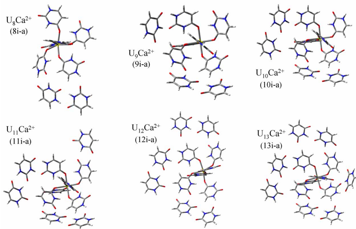
Figure S2. Proposed structures for U_nCa^{2+} with n = 8-13 .
