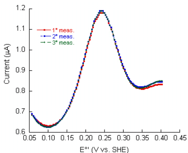
Fig. 1S Dfferential pulse voltammograms obtained at 4,4'-bipyridyl modified gold electrodes in three different solutions of cyt c in the presence of 0.2 M NaCl at 298K
