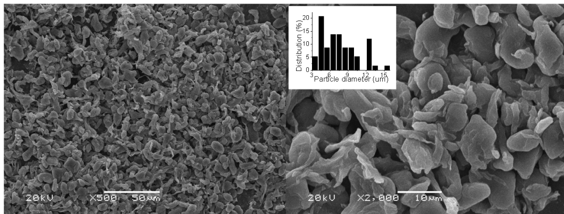
Fig. S1 SEM microscopy of PTFE particles (inset is the particle size distribution histogram).
